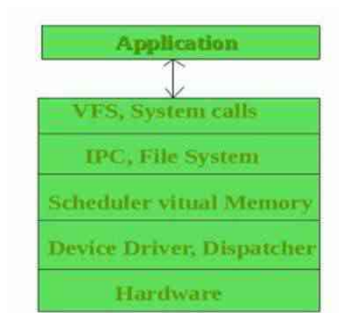
Figure 1.7.4 Monolithic Kernel
