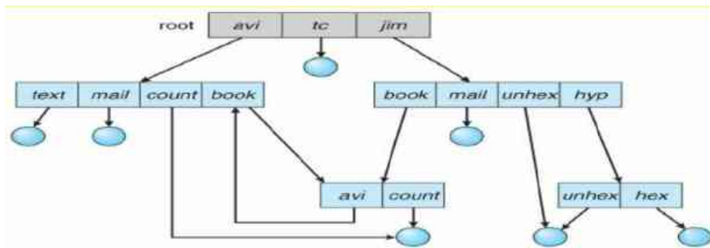
Figure - General graph directory.
