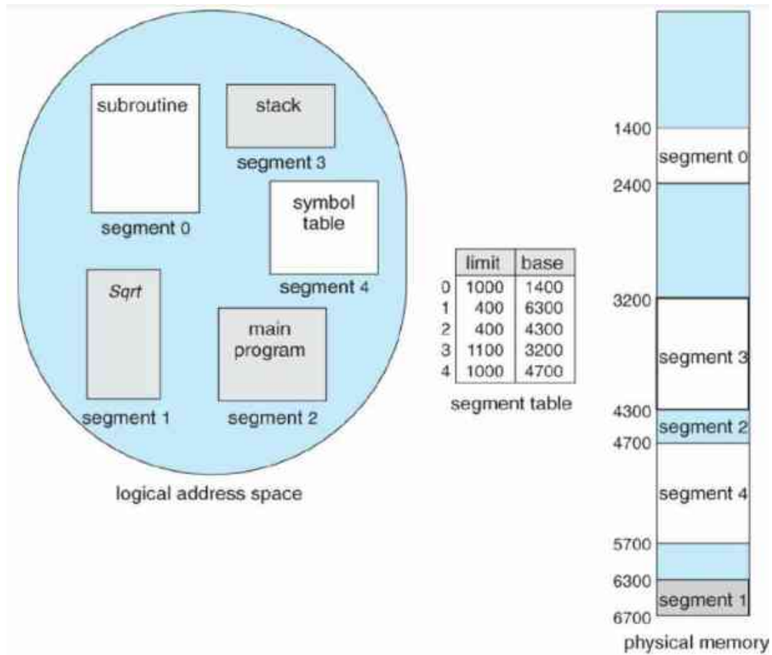
Figure - Example of segmentation
