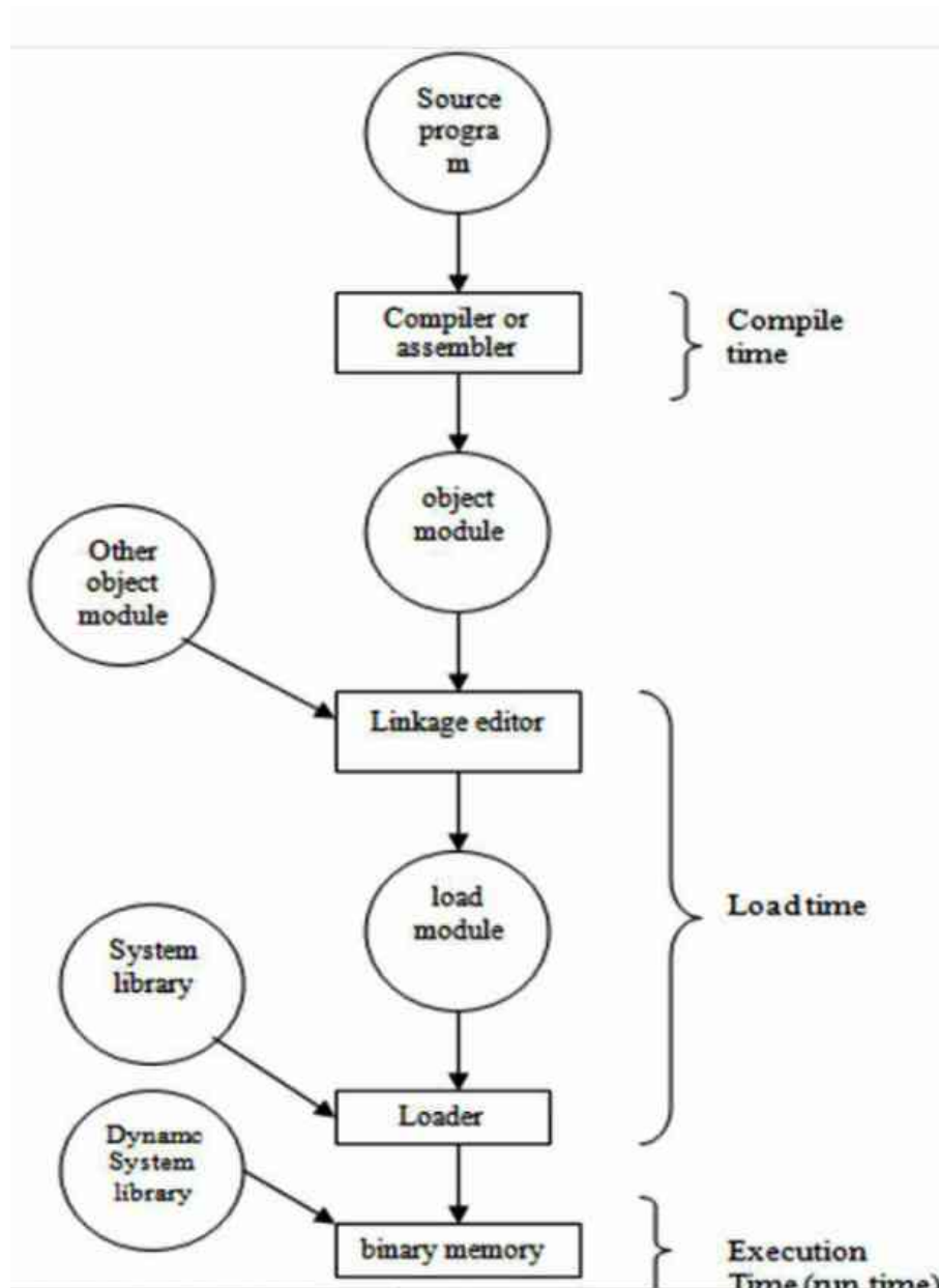
Figure - Multistep processing of a user program
