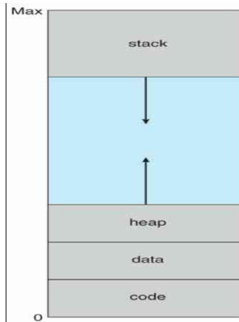
Figure 5.2 - Virtual address space
