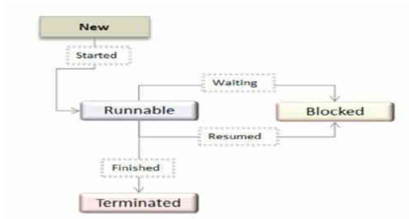
Figure Thread State Diagram
