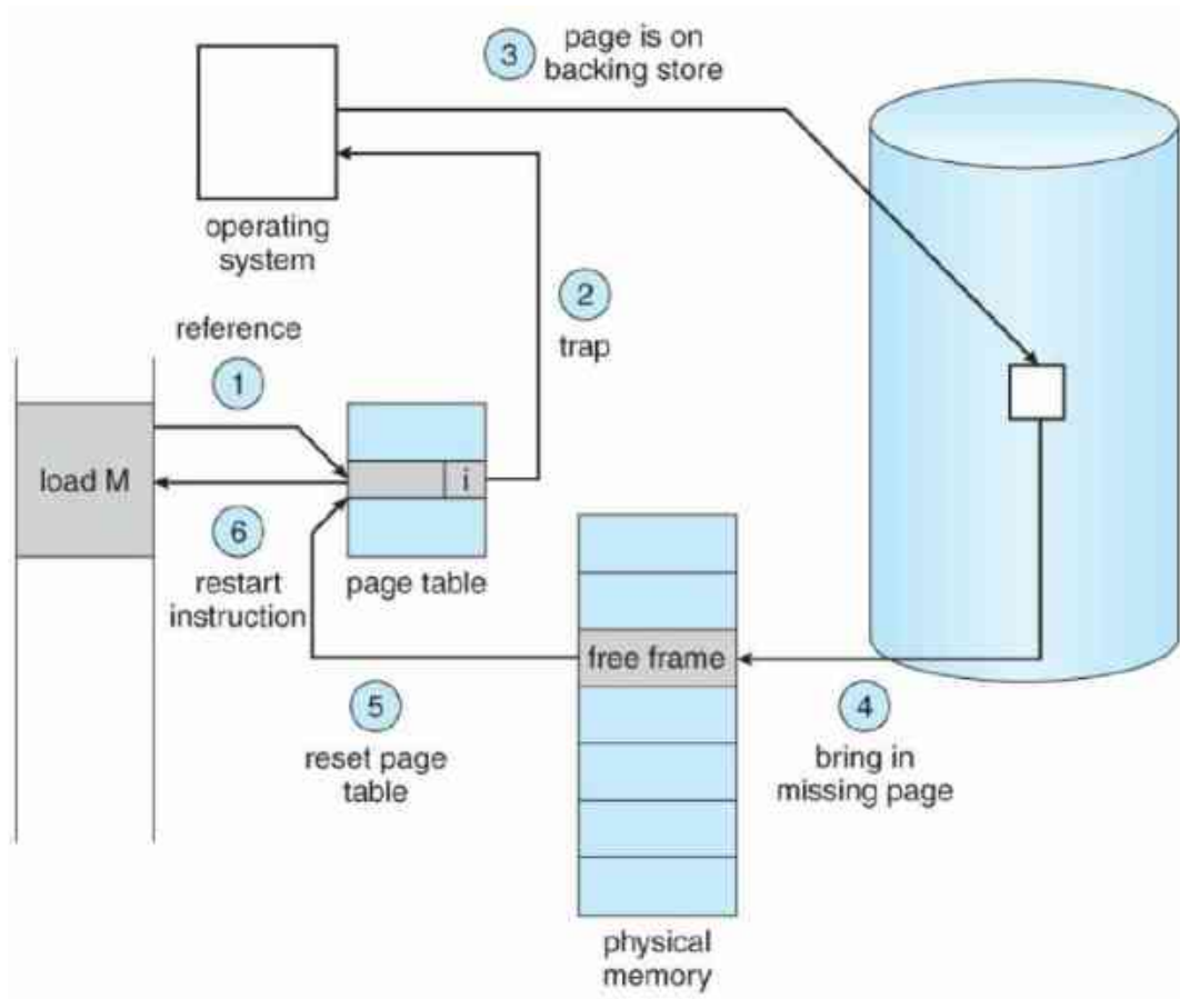
Figure 5.6 - Steps in handling a page fault
