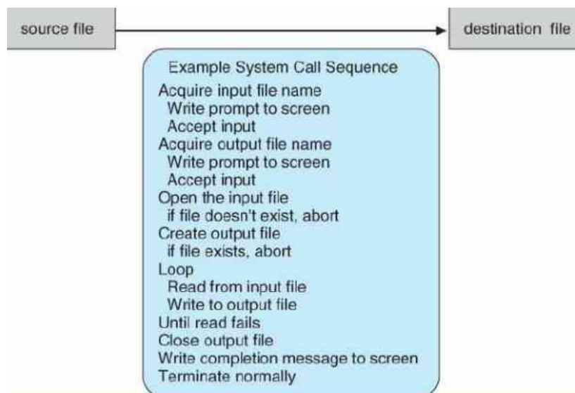
Figure 1.5 - Example of how system calls are used.
