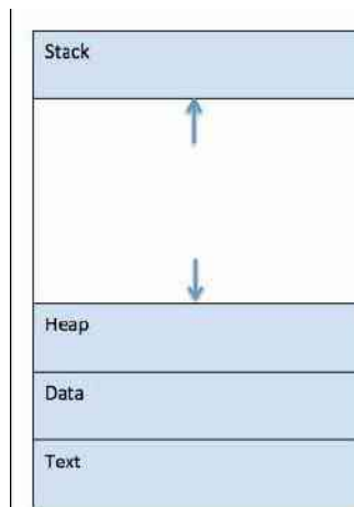
Figure2.1 Process
