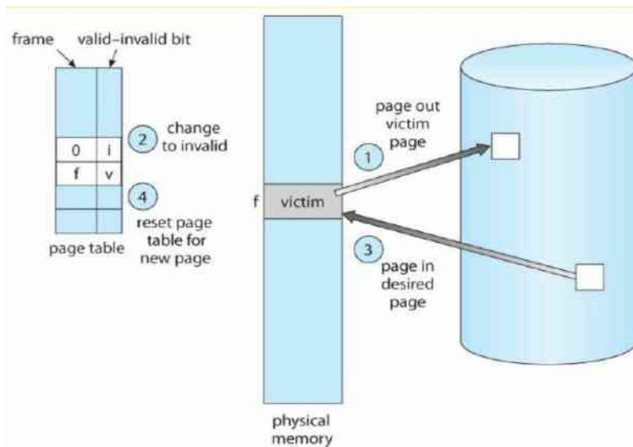
Figure 5.8 - Page replacement.
