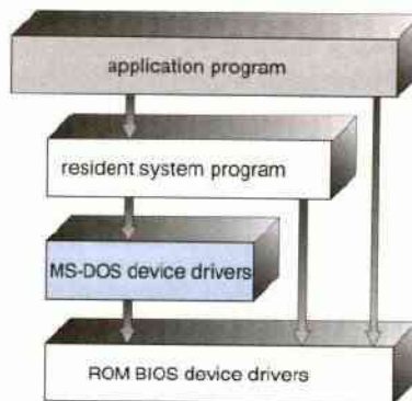
Figure 1.7.1 MS-DOS Structure
