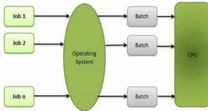
Figure1.3 Batch Processing
