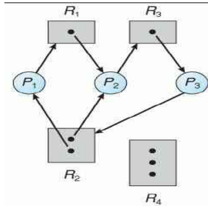
Figure Resource Allocation Graph with a deadlock
