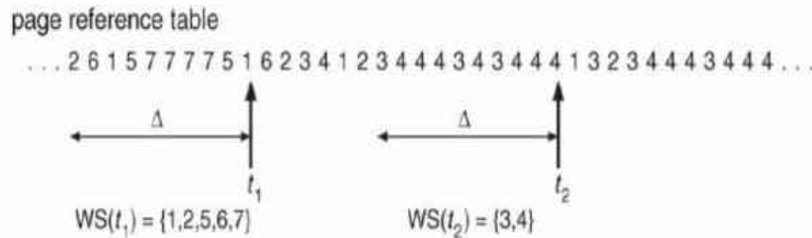
Figure 5.11 - Working-set model.
