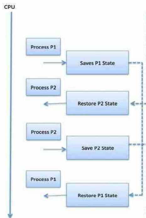
Figure 2.5 Context Switching
