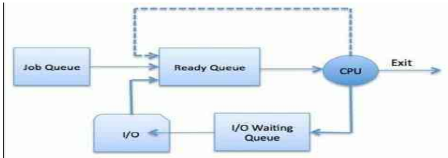
Figure 2.4 Process Scheduling Queues
