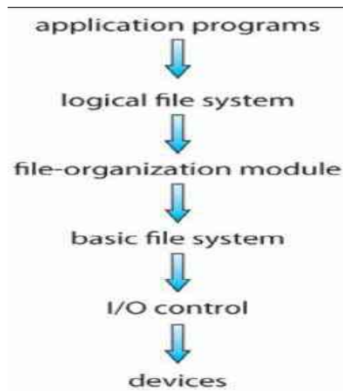
Figure - Layered file system.
