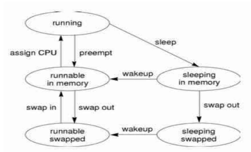
Figure Process State Transition Diagram
